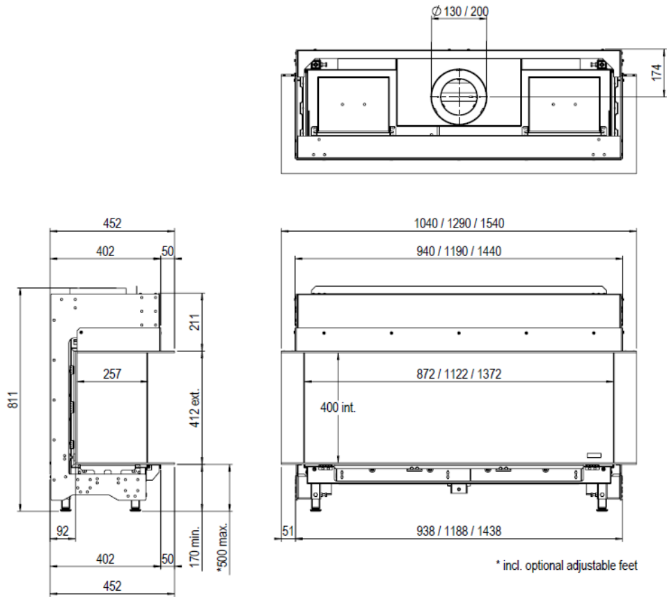
Dimensional Drawing MatriX 800-1050-1300/400 III
