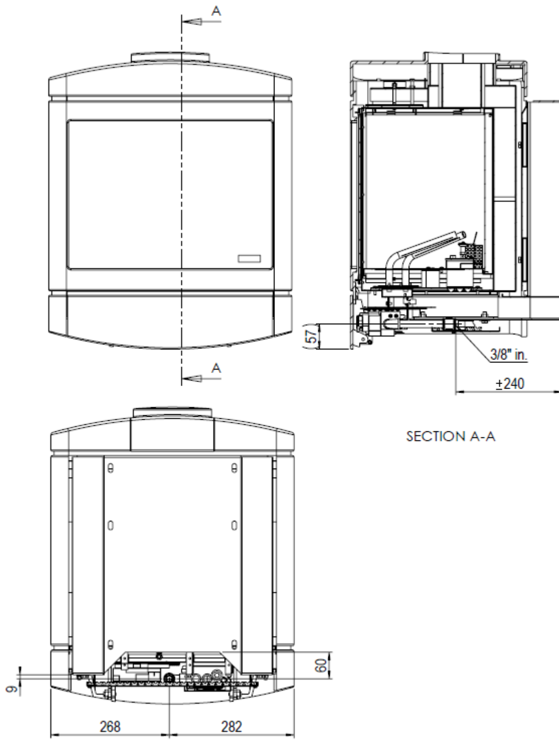
Dimensional Drawing gas connection Skive GV60
