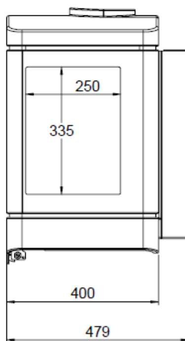
Dimensional Drawing Skive
