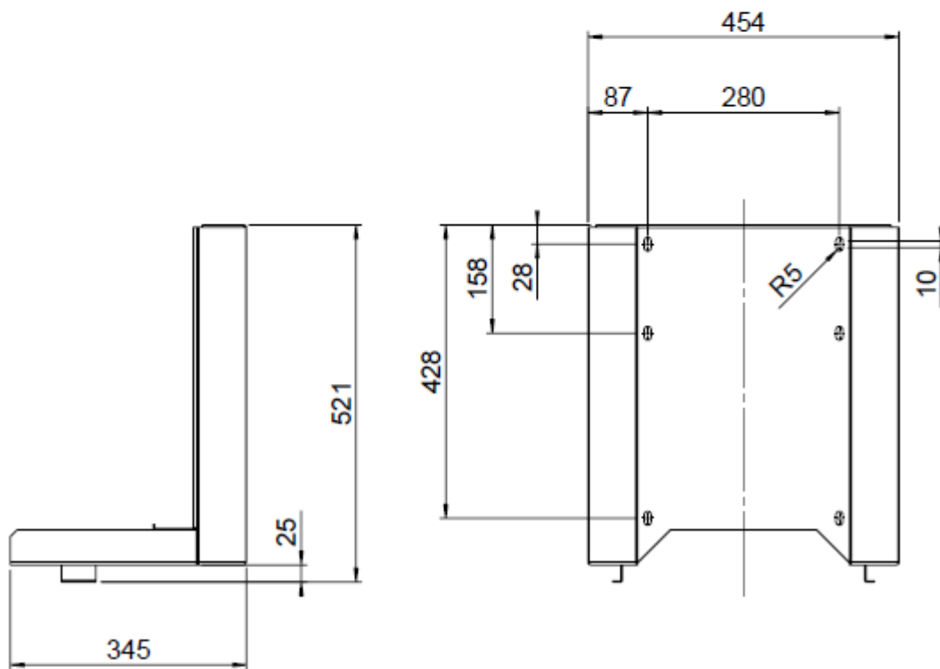
Dimensional Drawing wall support Skive
